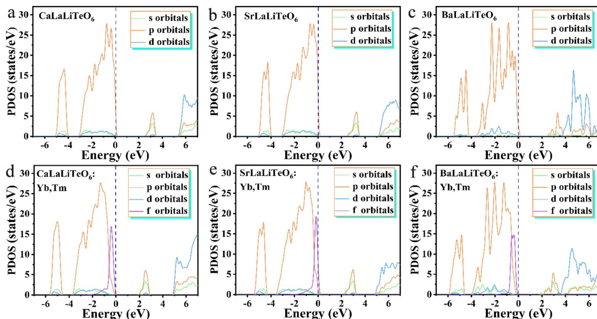
Fig. 5 The PDOS, bonding and anti-bonding orbitals of (a–c) \text{ALaLiTeO}_6 and (d–f) \text{ALaLiTeO}_6:\text{Yb,Tm} with (A = Ca, Sr, and Ba).
