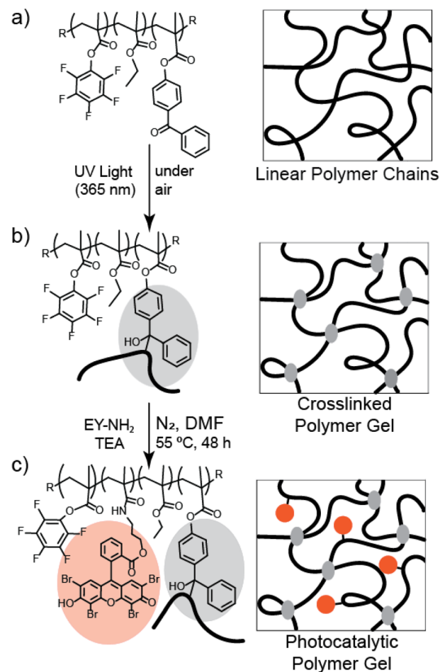
Fig. 1 (a) The chemical structure of the synthesized P(EtMA- co -BPMA- co -PFPMA) copolymer. R groups represent the variety of chain ends produced from free radical polymerization. (b) The terpolymer was treated with UV light ( \lambda_{\text{max}} = 365 \text{ nm} ) to crosslink the polymer via C,H-insertion chemistry. (c) Treatment with a primary amine-bearing photocatalyst (Eosin Y; EY-NH 2 ) in presence of triethylamine (TEA) substituted the pentafluorophenyl moieties to yield the final photocatalytic cross-linked network.
