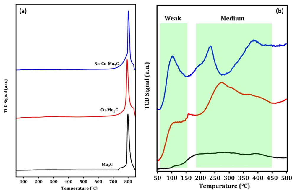
Fig. 4 \text{CO}_2 TPD analysis of the derived catalysts (a) and below 500 °C (b).
