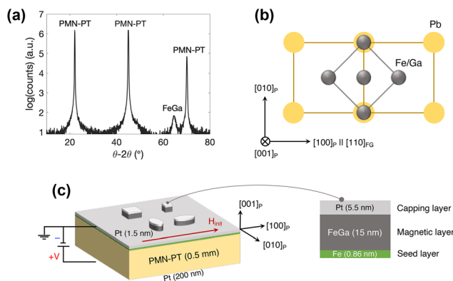
Fig. 1 (a) Ex situ XRD \theta – 2\theta scan of the multiferroic heterostructure composed of epitaxial (001) Fe–Ga and (001)-oriented PMN–PT. (b) Top-view schematic of the crystallographic orientation of the Fe–Ga cell (grey) with respect to the PMN–PT cell (yellow) (O, Mn, Nb and Ti atoms have been omitted for simplicity). The easy axis of Fe–Ga [110]_{\text{FG}} is aligned with the [100]_{\text{P}} direction of PMN–PT and the Fe–Ga [001]_{\text{FG}} axis is oriented out of plane. (c) Schematic description of the investigated multiferroic system. The PMN–PT has the [001]_{\text{P}} direction parallel to the surface normal, along which voltage is applied. After patterning, the magnetic microstructures are initialized by an external magnetic field, \mu_0 H_{\text{init}} \approx 250 \text{ mT} , applied in the direction as indicated by the red arrow. The multi-layered stack of the microstructures is zoomed in on the right.
