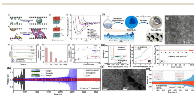
Fig. 4 (a) Schematic diagram of the agglomeration of Sn nanoparticles during cycling; (b) schematic diagram of the SnO 2 -induced deposition of the Na metal; (c) definition of W_{ag} ; (d) relationship between W_{sep} and distance; (e) voltage–capacity curves of the Na metal on different substrates and (f) the corresponding Na nucleation overpotentials; (g) changes in the nucleation overpotentials of rGO, Sn@rGO, and SnO 2 @rGO with the number of cycles; (h) plating–stripping curve of the NaF/SnO 2 @rGO anode at 0.5 mA cm -2 ; and (n) morphologies of SnO 2 (left) and Sn (right) nanoparticles after cycling. Reproduced with permission from ref. 66 Copyright 2020, Elsevier. (i) Schematic diagram of the preparation process of At-Sn@HCN; (j) schematic diagram of the morphology of At-Sn@HCN; (k) voltage–capacity curve of At-Sn@HCN at 2 mA cm -2 ; (l) nucleation overpotentials of Sn@HCN at different current densities; (m) CEs of At-Sn@HCN at different areal capacities; and (o) plating–stripping curve of the At-Sn@HCN/Na anode at 1 mA cm -2 –1 mA h cm -2 . Reproduced with permission from ref. 67 Copyright 2022, AAAS.
