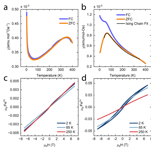
Fig. 6 Magnetic susceptibility data at 500 Oe of (a) bulk and (b) exfoliated KFeS 2 . The exfoliated KFeS 2 zero-field-cooled data (ZFC) has been fit as an Ising chain, shown in black. Field-dependent magnetization data of (c) bulk and (d) exfoliated KFeS 2 is also shown; note the hysteresis at T = 2 K that occurs only in the exfoliated sample. Additional data shown was collected at possible temperatures of interest: T = 85 K (broad peak) and T_N = 250 K.
