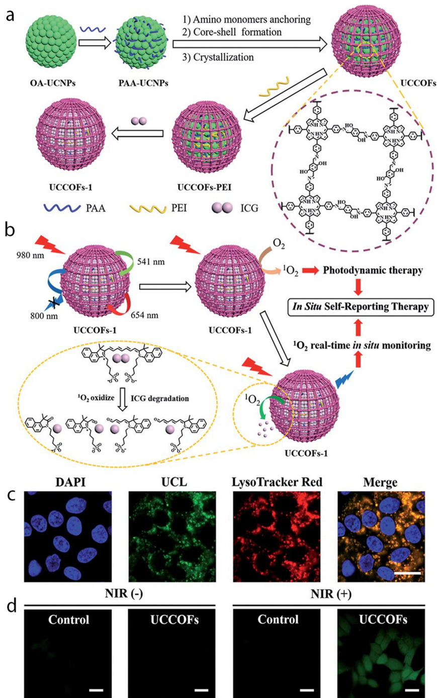
Fig. 10 (a) A schematic illustration showing the design and synthesis of the upconverting COF nanoplatfom UCCOFs-1. (b) A schematic illustration of the NIR-excited in situ self-reporting PDT process. (c) Confocal fluorescence images of HeLa cells treated with UCCOFs; scale bar: 20 \mu m . (d) Intracellular ^1O_2 production with or without NIR irradiation determined via a H2DCFH-DA assay; scale bar: 20 \mu m . Reproduced from ref. 92 with permission from the Royal Society of Chemistry.
