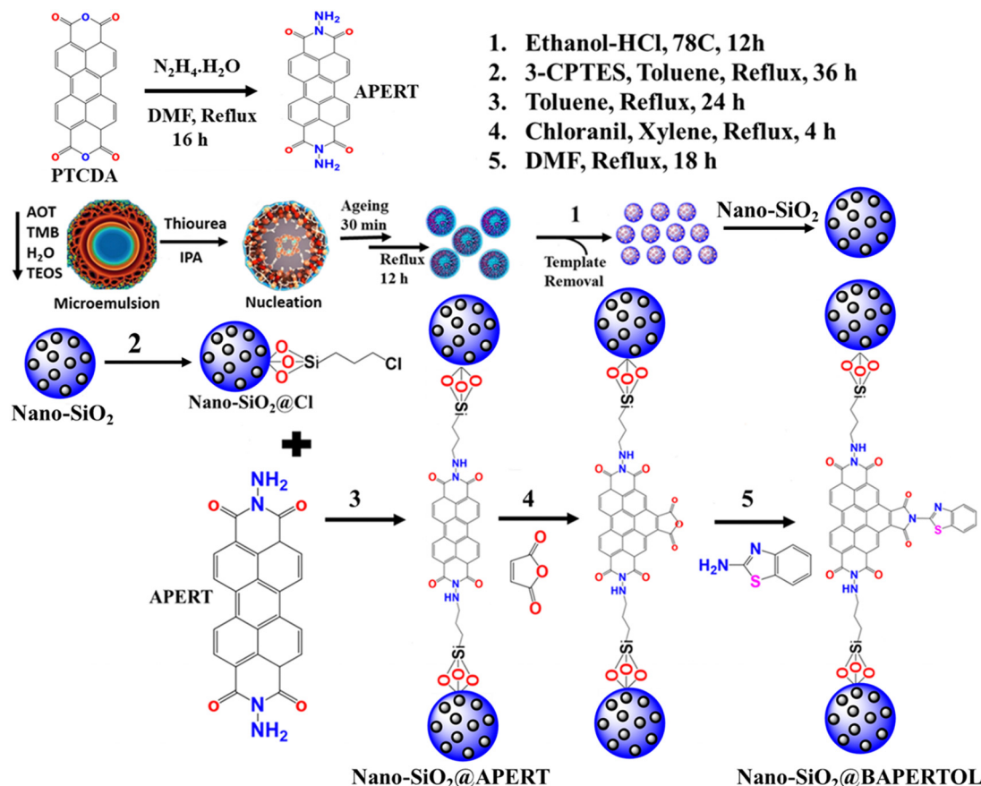
Scheme 1 The synthetic and chemical processing representation of the nano-silica ( \text{nano-SiO}_2 ), \text{nano-SiO}_2@\text{Cl} , \text{nano-SiO}_2@\text{APERT} , and the final material \text{nano-SiO}_2@\text{BAPERTOL} .
