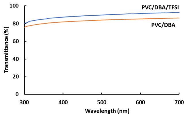
Fig. 1 Total transmittance of the PVC/DBA/TFSI and PVC/DBA gels.
