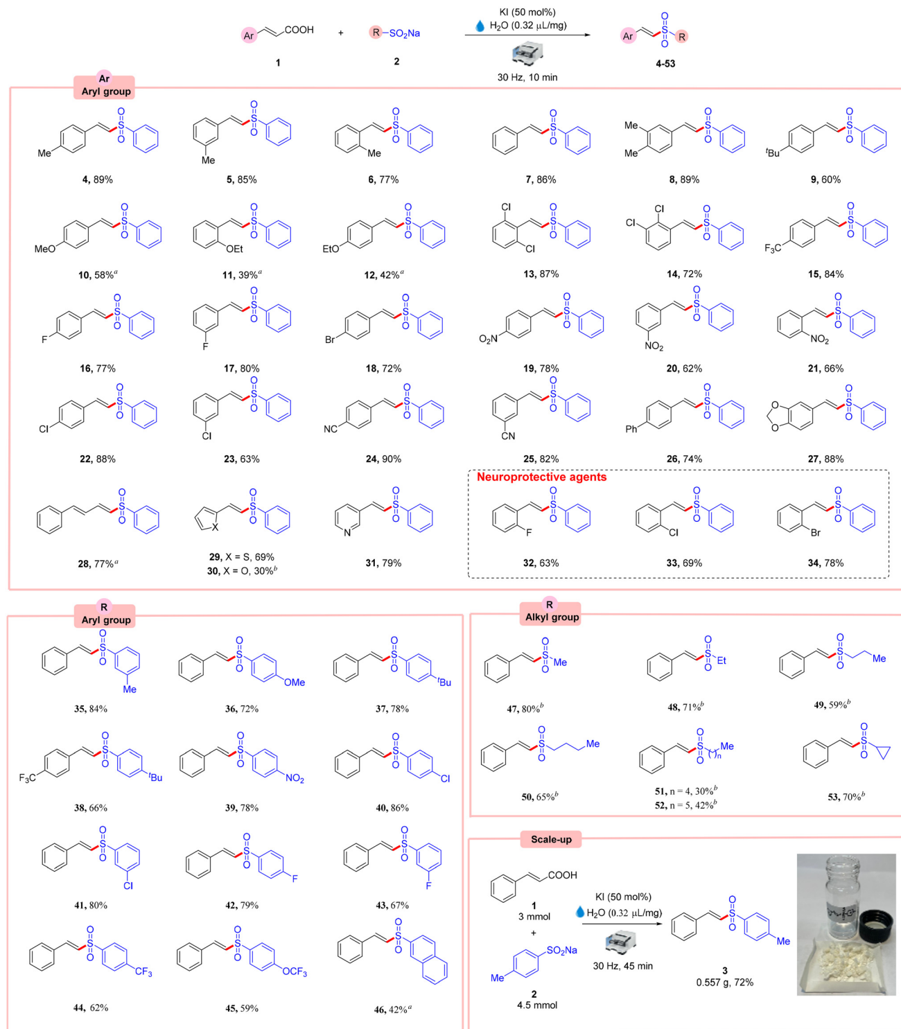
Scheme 2 Substrate scope for the decarboxylative sulfonylation reaction. Reaction conditions: aryl \alpha,\beta -unsaturated carboxylic acid 1 (0.5 mmol), sodium sulfonate 2 (0.75 mmol), KI (50 mol%), and \text{H}_2\text{O} ( \eta = 0.32 \mu\text{L mg}^{-1} ). The reaction was milled using a 10 mL Retsch stainless steel jar for 10 min at 30 Hz frequency with 5 mm, 2.5 g stainless steel grinding balls (5 \times 5 mm grinding balls) at room temperature. a 30 min, 30 Hz. b 40 min, 30 Hz.
