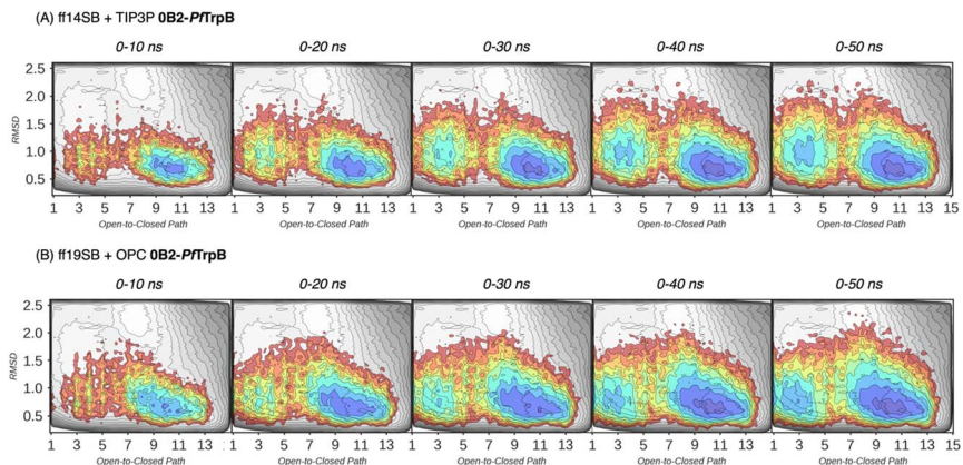
Fig. 4 Estimated FEL of OB2-PflTrpB . The estimated FEL from the accumulated multiple replica nanosecond timescale MD simulations performed starting at the ensemble of template-based AF2 predictions, is shown in colour on top of the previously reconstructed FEL of the PflTrpB variant (shown in grey scale). 19 FELs are displayed every 10 ns of MD simulation time and using two different combinations of forcefield and water model: (A) ff14SB and TIP3P water, and (B) ff19SB and OPC water. The x axis denotes the ensemble of structures generated from X-ray data for the open-to-closed transition of the COMM domain, which ranges from 1–5 (open, O), 6–10 (partially closed, PC), to 11–15 (closed, C), the y axis is the mean square deviation (MSD, in Å 2 ) from the path of O-to-C structures generated. Most stable conformations are shown in blue, whereas higher energy regions are shown in red.
