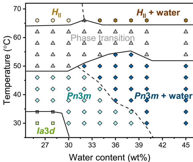
Fig. 2 Phase diagram of the monolinolein–water mesophase as a function of water content and temperature obtained by SAXS. Phase labels: Ia3d , green squares; Ia3d + Pn3m , grey squares; Pn3m , light blue diamond; Pn3m + water, dark blue diamond; phase transition, grey up-pointing triangles; H II , light yellow hexagons; H II + water, dark yellow hexagons. The lines dividing the phase regions are a guide to the eye. A dashed line separates the mesophases with and without excess water.
