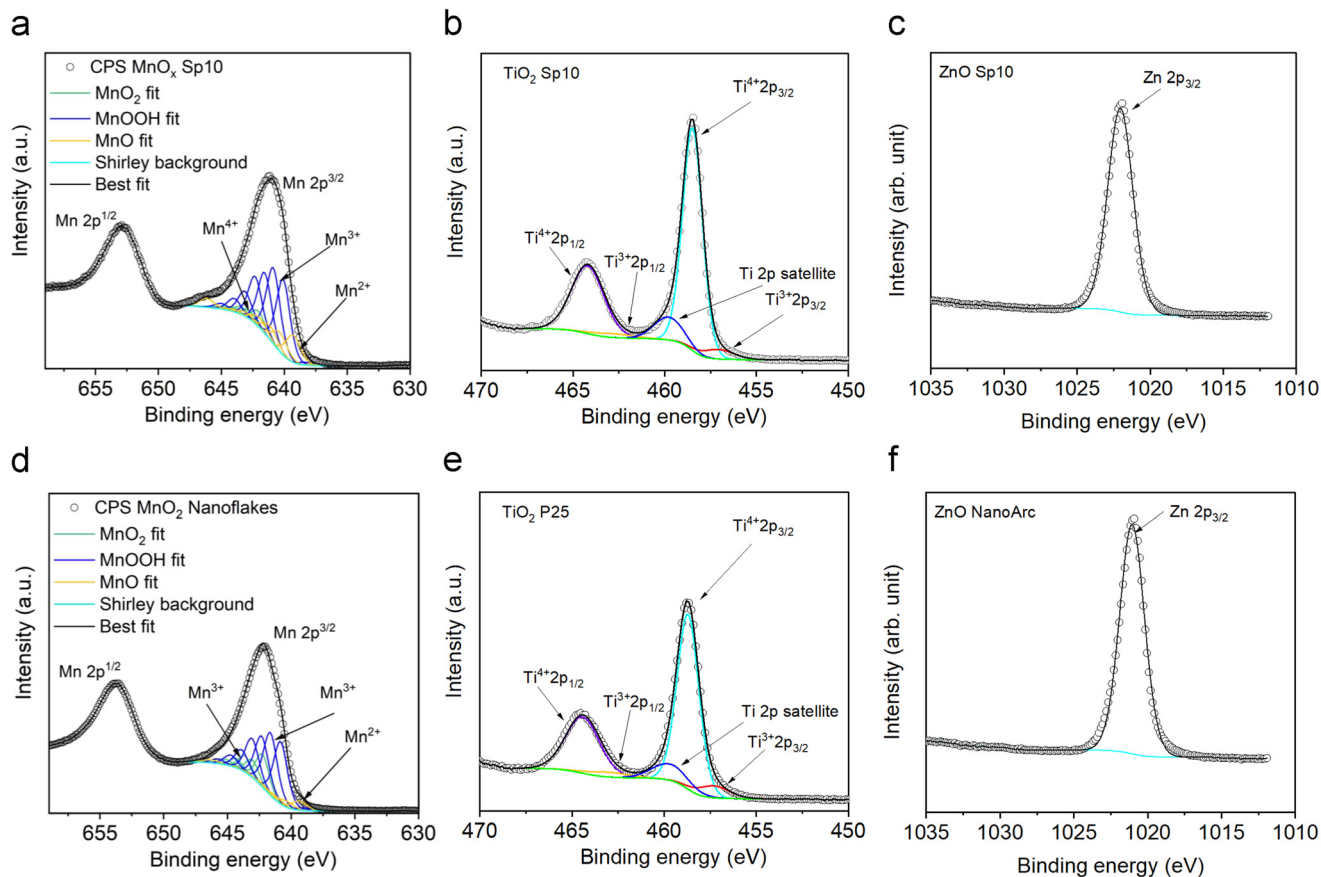
Fig. 10 High-resolution a) Mn 2p, b) Ti 2p, and c) Zn 2p XPS spectra of spark-ablated manganese oxide ( \text{MnO}_x ), titanium dioxide ( \text{TiO}_2 ), and zinc oxide (ZnO) nanoparticles, respectively, and the comparison with the XPS spectra of d) sol-gel prepared \text{MnO}_2 and commercial e) \text{TiO}_2 P25 and f) ZnO NanoArc. Peak deconvolution indicates the oxidation states of the material.
