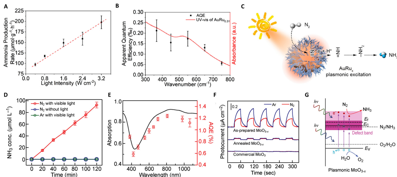
Fig. 7 (A) and (B) Photocatalytic ammonia production rates and calculated AQEs by \text{AuRu}_{0.31} . (C) The schematic diagram for the photo driven \text{NH}_3 synthesis over the \text{AuRu}_{0.31} nanostructure. These figures have been reproduced from ref. 118 with permission from American Chemical Society, copyright 2019. (D) Photothermal catalytic \text{NH}_3 production of \text{MoO}_{3-x} under different conditions. (E) Action spectrum of the \text{MoO}_{3-x} spheres for \text{N}_2 photo-fixation. (F) Photocurrent responses of serial \text{MoO}_{3-x} spheres under an Ar and \text{N}_2 atmosphere, respectively. (G) Schematics illustrating the band structures of the plasmonic \text{MoO}_{3-x} photocatalyst. These figures have been reproduced from ref. 121 with permission from John Wiley & Sons, copyright 2021.
