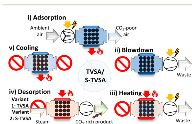
Fig. 3 The five phases of a temperature vacuum swing adsorption cycle (TVSA) and a steam-assisted temperature vacuum swing adsorption cycle (S-TVSA) applied for DAC are adapted from Young et al. and Stampi-Bombelli et al. 31,35 (i) Adsorption: a fan blows ambient air through the adsorption column; CO 2 and H 2 O are adsorbed. (ii) Blowdown: a vacuum pump decreases the column pressure to desorption pressure as the column inlet is closed. (iii) Heating: a jacket heats the column to the desorption temperature. (iv) Desorption via the TVSA cycle: extraction of CO 2 with closed column inlet; desorption via the S-TVSA cycle: extraction of CO 2 by injecting superheated steam. (v) Cooling: cooling of the adsorption column to below 90 °C.
