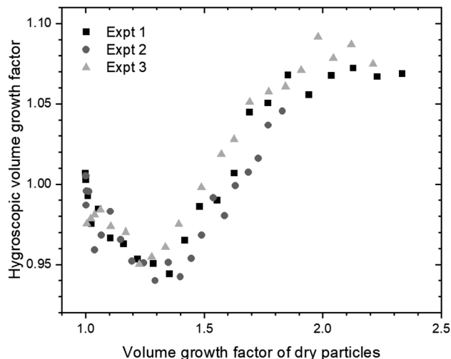
Fig. 2 Hygroscopic volume growth factor as a function of the volume growth factor of the dry particles, a measure of the SOA coating volume, for three experiments with initially 250 nm nanoplastics, illustrating intra- and inter-experiment variability. There is more scatter in the hygroscopic volume growth factor than in the individual time series of diameter growth factors, because the hygroscopic volume growth factor is a measure of the small difference between these time series.
