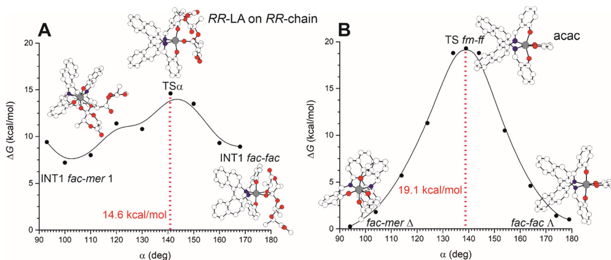
Fig. 4 Free energy profiles of the transformation from fac-mer \Delta to fac-fac \Delta for (R) -1 as a function of the O_L -Al- O_L valence bond. The reorganization path moving from TS1 ( fm1 ) to TS2 ( ff ) as a function of \alpha for RR -LA polymerization is reported in A. The analogous path by using the bidentate acac^- is reported in B. Aluminum, oxygen and nitrogen atoms in gray, red and blue. Hydrogen atoms have been omitted for clarity.
