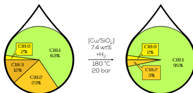
Fig. 19 Composition of the C18 fatty acid fraction in the selective hydrogenation of canola oil as performed by Zaccheria. 113
