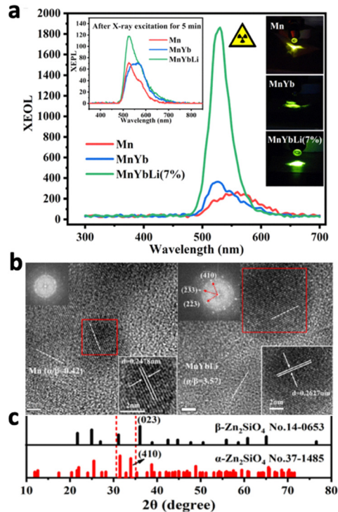
Fig. 19 (a) X-ray excited luminescence spectrum and afterglow spectrum (inlet) of Mn, MnYb, and MnYbLi (7%) samples after X-ray excitation for 5 min. (b) High resolution TEM images of Zn 2 SiO 4 :Mn ( \alpha/\beta = 0.42 , left) and Zn 2 SiO 4 :Mn,Yb,Li ( \alpha/\beta = 3.57 , right) samples. (c) XRD patterns of \alpha -Zn 2 SiO 4 and \beta -Zn 2 SiO 4 . Reproduced with permission from ref. 210. Copyright 2023, American Chemical Society.
