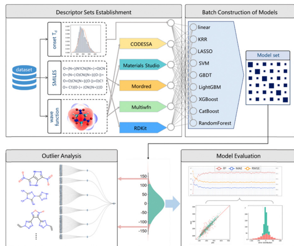
Fig. 15 The workflow of T_d prediction. Four sections are involved, including descriptor set establishment, batch construction of models, model evaluation, and outlier analysis. Reproduced with permission from ref. 115. Copyright 2024, Elsevier.
