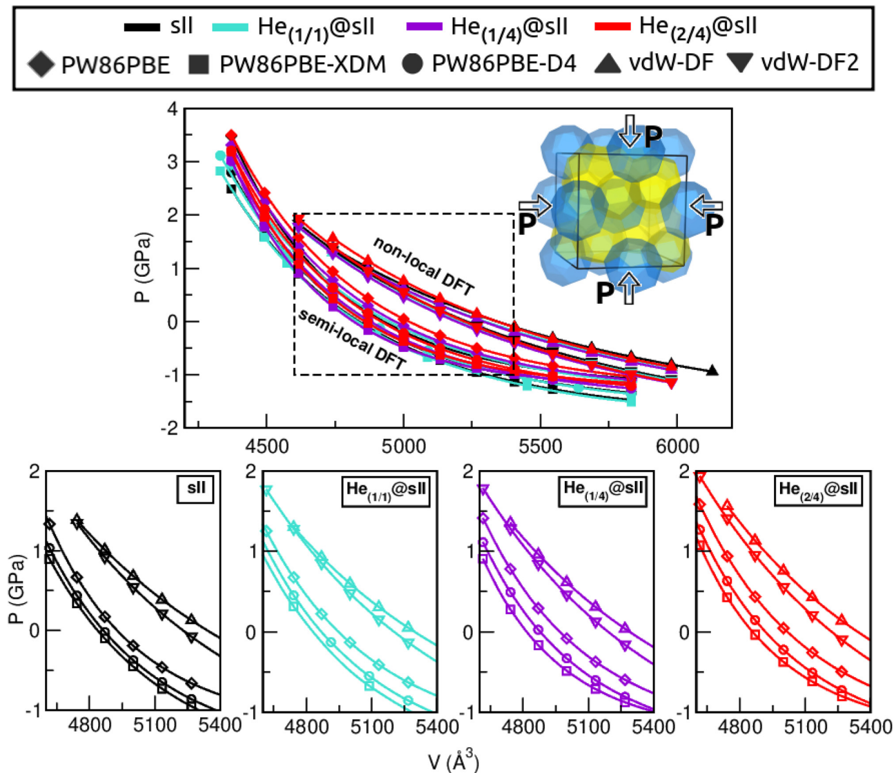
Fig. 5 Pressure effects on the volume, V (Å 3 ), assuming empty, single- and multiple-cage occupancy of both small and large cages of the sII crystal. The upper panel displays the combined results of semi-local and non-local functionals, while the lower panels present these outcomes individually for each crystal system.
