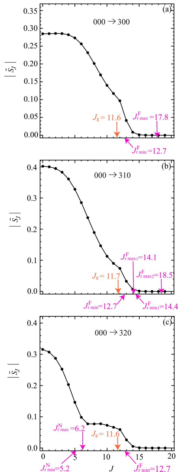
Fig. 1 Plots of |\tilde{S}_J| versus J at E_{\text{trans}} = 62.09 meV. The black solid circles are the numerical S matrix data, \{|\tilde{S}_J|\} , at integer values of J , which have been joined by straight lines. The orange arrow indicates the value of the glory angular momentum variable, J_g . The pink arrows indicate the values of the nearside (N) and farside (F) rainbow angular momentum variable. The notation and values of J_g , and the rainbow angular momenta, are taken from Fig. 6. The transitions are: (a) 000 \rightarrow 300, (b) 000 \rightarrow 310, (c) 000 \rightarrow 320.
