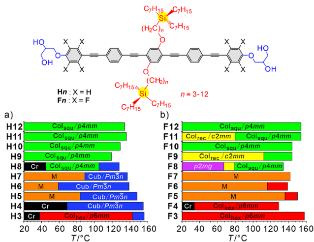
Fig. 2 Molecular structure and LC phases of (a) H n and (b) F n as observed on cooling with 10\text{ K min}^{-1} ; abbreviations: Cr = crystalline solid; Col hex / p6mm and Col sq / p4mm = triangular and square LC honeycombs, respectively; Col rec / c2mm and p2mg = tilings by rhombic and non-regular triangular honeycombs, respectively; Cub/ Pm\bar{3}n = cubic network phase with Pm\bar{3}n space group; M = unknown LC phases; isotropic liquid is at the right side of the columns; for numerical data, transitions on heating and enthalpies, see Table S1a, b, for DSCs Fig. S1 and S2, for textures Fig. S3–S6, for SAXS/WAXS data Fig. S7–S10, Tables S2–S29 (ESI † ).
