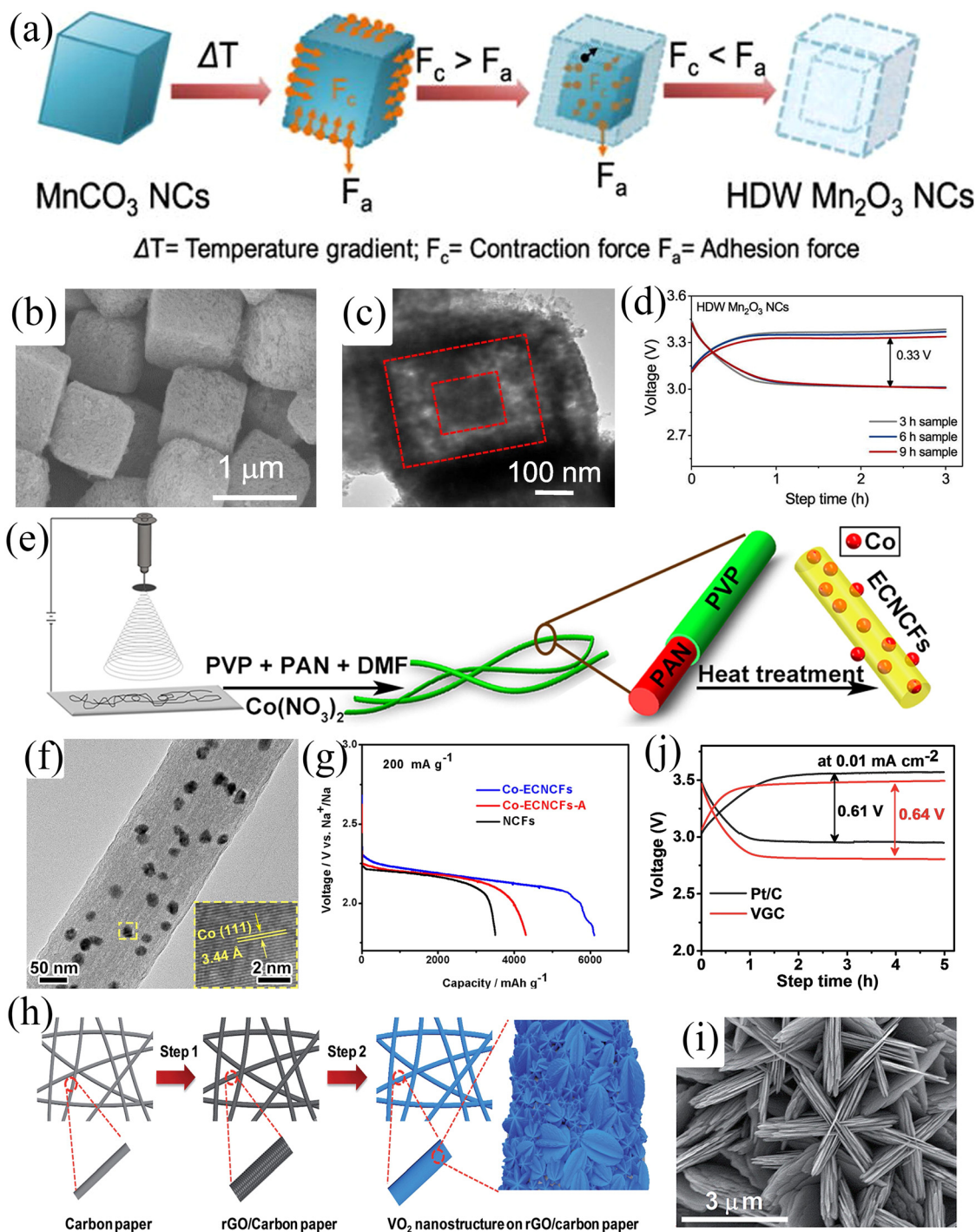
Fig. 9 (a) Schematic illustration of the synthesis of hollow double-walled Mn 2 O 3 nanocubes. (b) SEM and (c) TEM images of HDW Mn 2 O 3 NCs. (d) Galvanostatic charge/discharge profiles of SABs at a current density of 5.0 mA g -1 built-up by Mn 2 O 3 electrodes prepared via the hydrothermal method with different time intervals. (Reproduced from ref. 86 with permission from Elsevier). (e) Schematic illustration of the synthesis of Co-ECNCFs. (f) TEM image of Co-ECNCFs (inset: HRTEM image and the (110) lattice plane of Co particles). (g) Galvanostatic discharge curves at a current density of 200 mA g -1 with different electrodes. (Reproduced from ref. 27 with permission from Elsevier). (h) Schematic illustration of the synthesis of VGC. (i) SEM image of VGC. (j) The charge-discharge profiles of the assembled SABs using VGC and Pt/C electrodes at a current density of 0.01 mA cm -2 . (Reproduced from ref. 88 with permission from the Royal Society of Chemistry).
