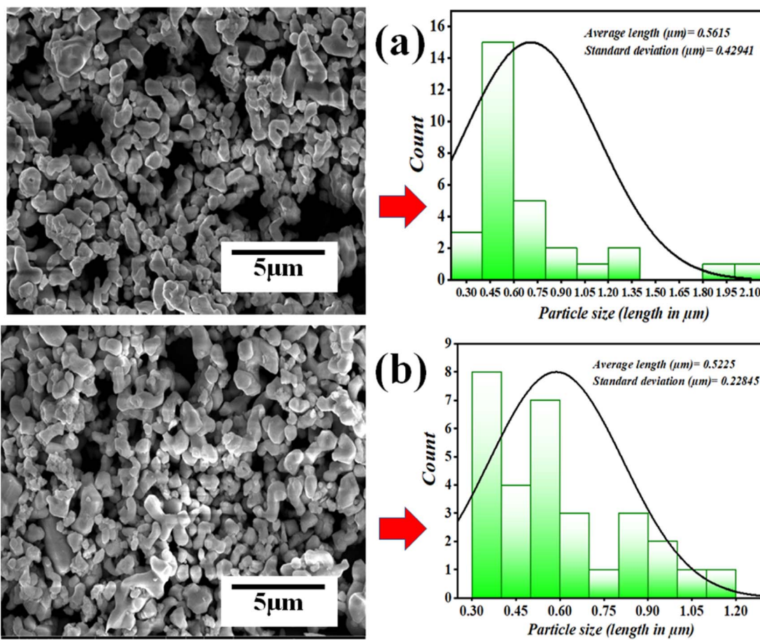
Fig. 11 SEM micrographs depicting particle size (a) before ball milling, (b) after ball milling.
