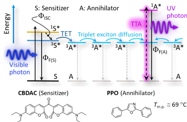
Scheme 1 Schematic energy diagram of TTA-UC in this study. X, 1X^* , and 3X^* (X = S: sensitizer or A: annihilator) denote the ground state, excited singlet state, and excited triplet state, respectively. TET: triplet energy transfer; TTA: triplet–triplet annihilation. Bottom shows the sensitizer and annihilator selected in this study.
