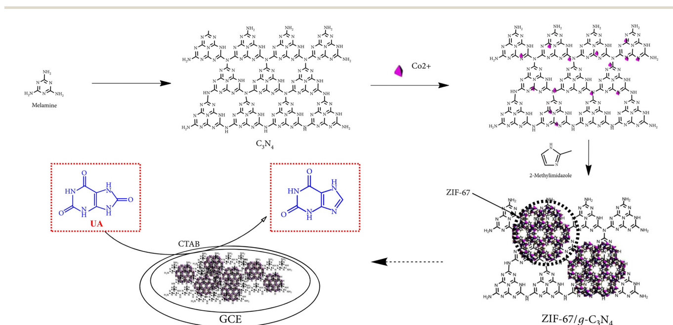
Fig. 2 Reaction mechanism of UA oxidation at the ZIF-67/g-C 3 N 4 -modified electrode. Reproduced with permission from ref. 128. Copyright (2020) Hindawi.
