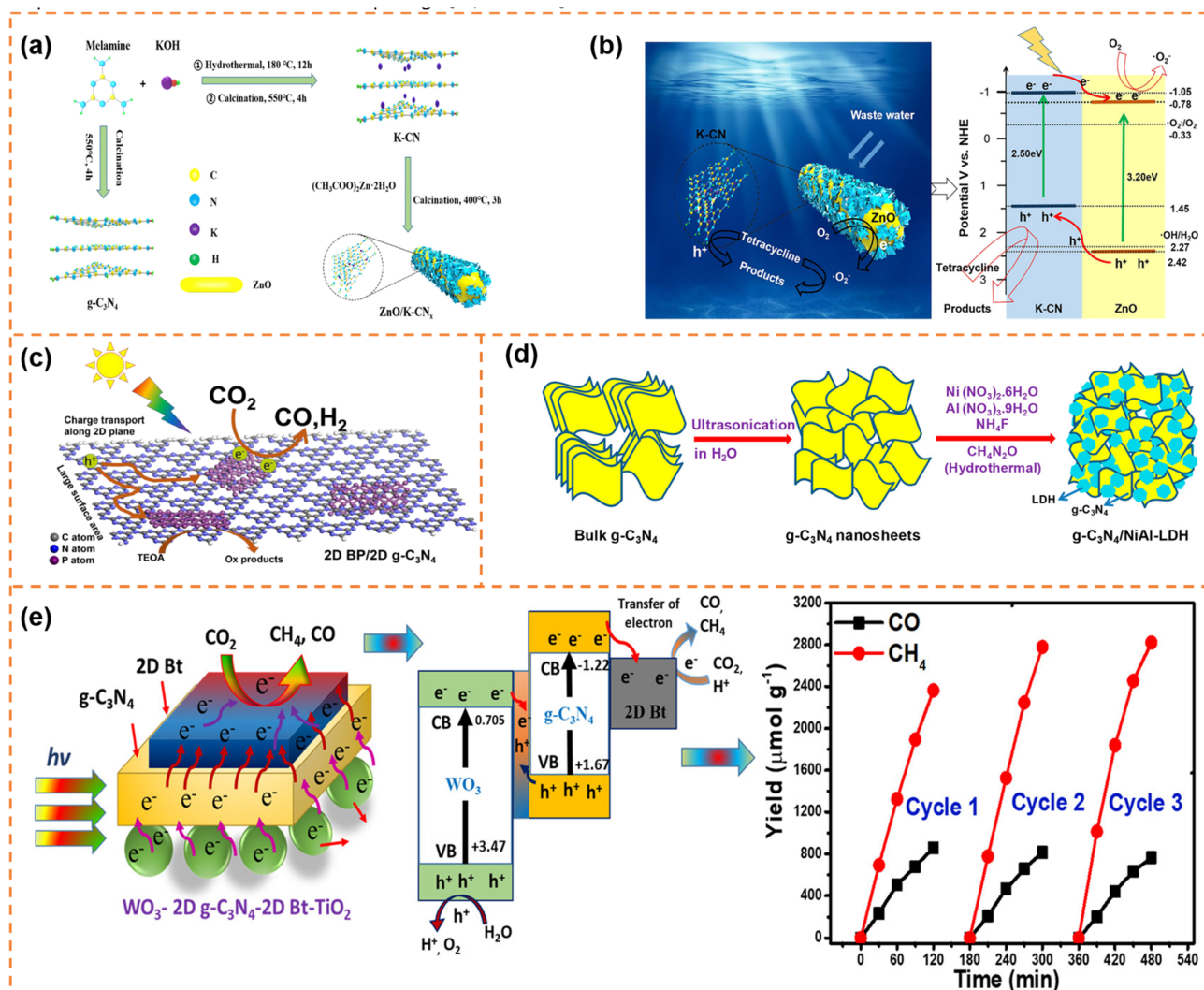
Fig. 12 (a) Schematic diagram of the synthesis and assembly route of photocatalyst materials. (b) Schematic diagram of the charge separation and photocatalytic mechanism of type-II \text{ZnO/K-CN}_{0.5} heterojunctions under simulated sunlight. Reprinted with permission from ref. 166, © American Chemical Society 2020. (c) Illustration of the photocatalytic mechanism of the 2D BP/2D g\text{-C}_3\text{N}_4 system under visible-light irradiation. Reprinted with permission from ref. 169, © Elsevier B.V. 2020. (d) Schematic illustration of the synthesis process of g\text{-C}_3\text{N}_4/\text{NiAl-LDH} hybrid heterojunctions. Reprinted with permission from ref. 170, © American Chemical Society 2018. (e) Proposed mechanism and stability analysis of photocatalytic \text{CO}_2 reduction with \text{H}_2\text{O} over the Bt-mediated \text{WO}_3/g\text{-C}_3\text{N}_4 composite under visible-light irradiation. Reprinted with permission from ref. 172, © American Chemical Society 2020.
