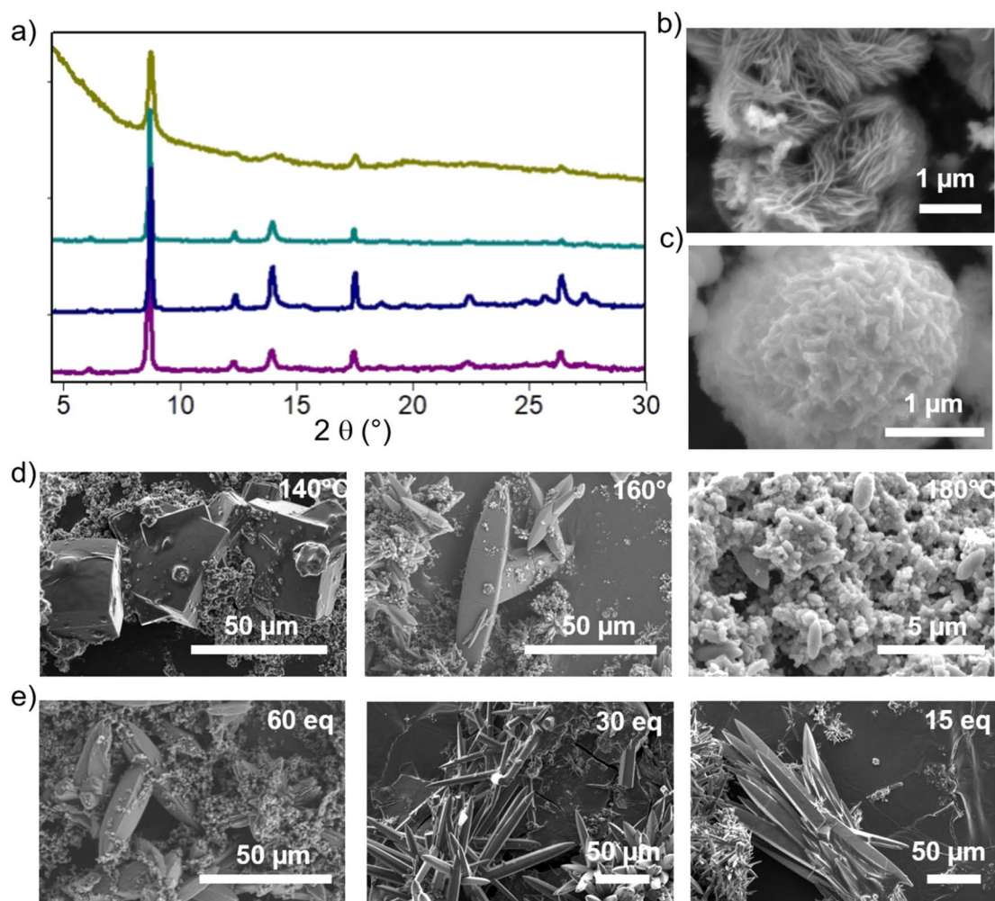
Fig. 2 (a) PXRD patterns from top to bottom: CatPMOF-1(Fe) (synthesis at 160 °C) and CatPMOF-1(Fe)-pz synthesized at 140 °C, 160 °C and 180 °C. SEM images of (b) Ni-CatPMOF-1(Fe); (c) CatPMOF-1(Fe); (d) the crystal size and morphological evolution of CatPMOF-1(Fe)-pz as a function of temperature with synthesis parameters H_{10}TcatPP/FeCl_3/pz/H_2cat = 1/3/3/60 , DMF/H_2O 1/4 and (e) as a function of the H_2cat modulator content at 150 °C.
