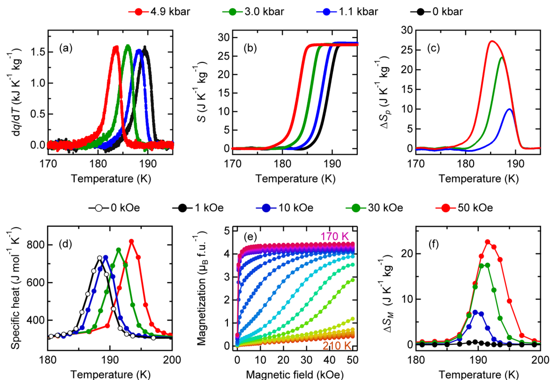
Fig. 4 (a) Heat flow curves divided by the cooling rate \text{dq/dT} , (b) corresponding entropy as a function of temperature, and (c) isothermal entropy changes of \text{BiCu}_3\text{Cr}_4\text{O}_{12} under various applied pressures. (d) Specific heat capacity curves under various magnetic fields, (e) isothermal magnetization as a function of applied field between 170 and 210 K, and (f) isothermal entropy changes obtained from the magnetization changes measured under magnetic fields from 0 to 50 kOe.
