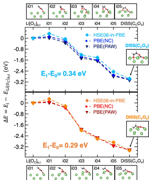
Fig. 4 VC migration on Li metal: minimum energy paths (MEPs) for the migration of the VC molecule from its adsorbed to dissociated states, (top) \text{DISS}(\text{C}_6\text{O}_V) and (bottom) \text{DISS}(\text{C}_V\text{O}_V) , computed by means of the CI-NEB approach. The corresponding energetics obtained at the DFT-PBE(PAW) (dark-blue and burgundy lines), DFT-PBE(NC) (blue and red lines) and DFET-HSE06-in-PBE (light-blue and orange lines) levels of theory are plotted along the MEPs. The related reaction intermediates (images i01-i05) are also displayed.
