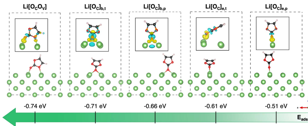
Fig. 1 VC adsorption on Li metal: minimum-energy structures of VC/ \text{Li}(001) adsorbed states in different configurations and corresponding adsorption energies calculated according to eqn (2) at the PBE-D3 level of theory. Insets: charge density difference plots computed according to eqn (3) (isosurface: 3 \text{meV} \text{ \AA}^{-3} ). Color code: Li (green), C (black), O (red), and H (white); electron gain (yellow) and electron loss (cyan).
