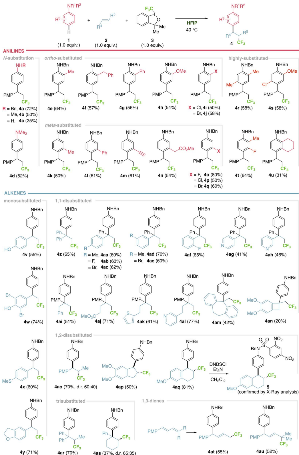
Fig. 2 Scope of the trifluoromethylarylation of alkenes using anilines in HFIP. General conditions: 0.2 mmol of aniline \mathbf{1} , 0.2 mmol of alkene \mathbf{2} and 0.2 mmol of \mathbf{3} in 0.5 mL of HFIP. PMP: para -methoxyphenyl. DNBSCl: 2,4-dinitrobenzenesulfonyl chloride.
