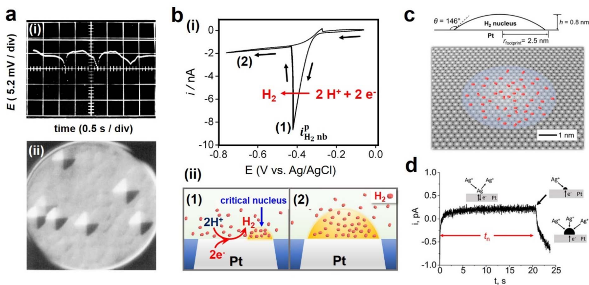
Fig. 2 (a) (i) E - t trace indicating overpotential fluctuation during two-dimensional nucleation of Ag at -65 \mu\text{A cm}^{-2} on a “defect-free” Ag(100) surface and (ii) growth pyramids on the flat Ag(100) plane. Adapted with permission from ref. 19; (b) the nucleation of H 2 nanobubble on a Pt electrode. (i) Cyclic voltammogram, and (ii) schematic illustration of bubble evolution showing (1) critical nucleus and (2) a steady-state H 2 bubble formation at a Pt nanoelectrode. Adapted with permission from ref. 35. Copyright 2019 American Chemical Society. (c) Schematic of the cross-section and 3D view of the critical H 2 nucleus. Adapted with permission from ref. 35. Copyright 2019 American Chemical Society. (d) i - t curve exhibiting the nucleation and the growth of a single Ag nanoparticle on a Pt nanoelectrode. Reprinted with permission from ref. 46. Copyright 2023 American Chemical Society.
