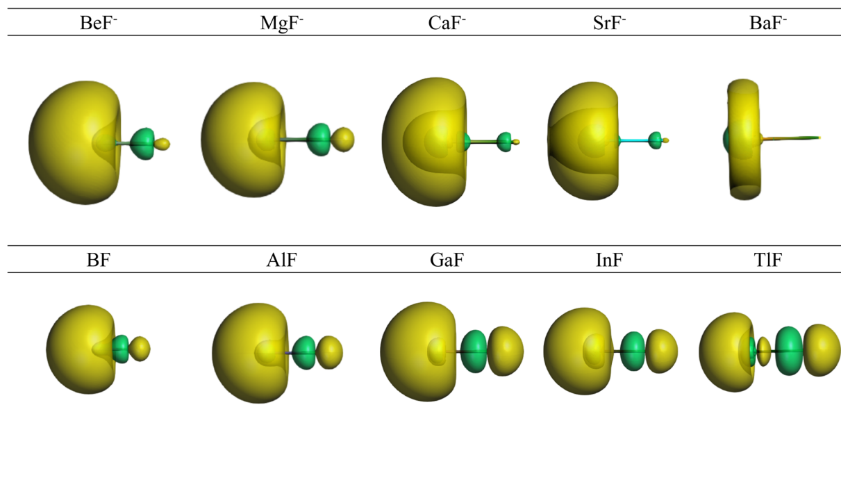
Fig. 1 Shape of the HOMO of \text{AeF}^- ( \text{Ae} = \text{Be–Ba} ) and \text{EF} ( \text{E} = \text{B–Tl} ). The \text{Ae/E} atoms are on the left side and the fluorine atom on the right.
