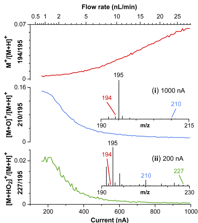
Fig. 5 Detection of caffeine molecular ion. Detection of caffeine (25 \mu\text{M} ) in 200 mM HCl under different spray currents. Red: Intensity ratio of \text{M}^+/\text{[M+H]}^+ . Blue: [\text{M}+\text{O}]^+/\text{[M+H]}^+ . Green: [\text{M}+\text{HO}_2]^+/\text{[M+H]}^+ . Mass spectra in the inset are taken at 1000 and 200 nA.
