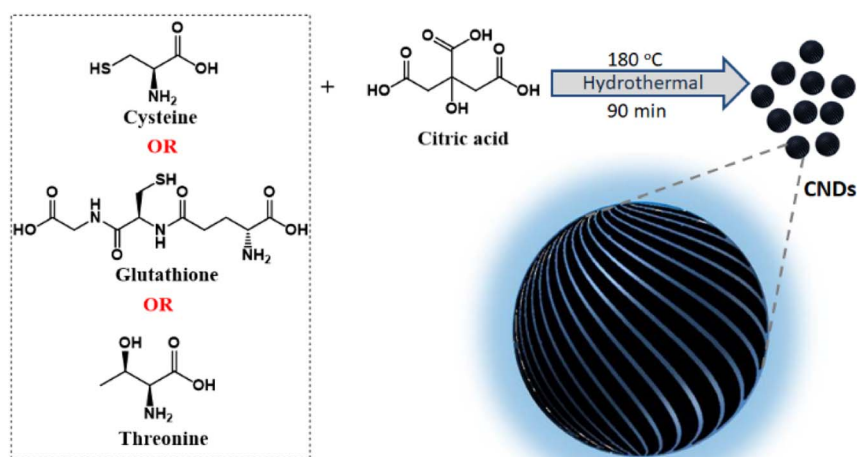
Fig. 1 Scheme illustrating the synthesis of chiral CNs using a combination of citric acid and different chiral agents as precursors.
