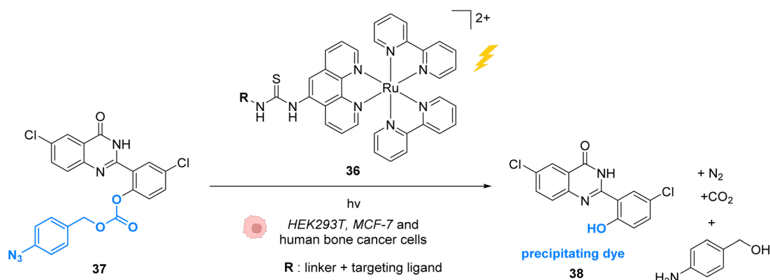
Fig. 14 Azide reduction of a pro-fluorescent probe inside different cell lines by the ruthenium(II) complex 36 , which is conjugated with a protein linker R, allowing specific localisation of the reaction in targeted parts of the cell by two-photon excitation at 730 nm. 50
