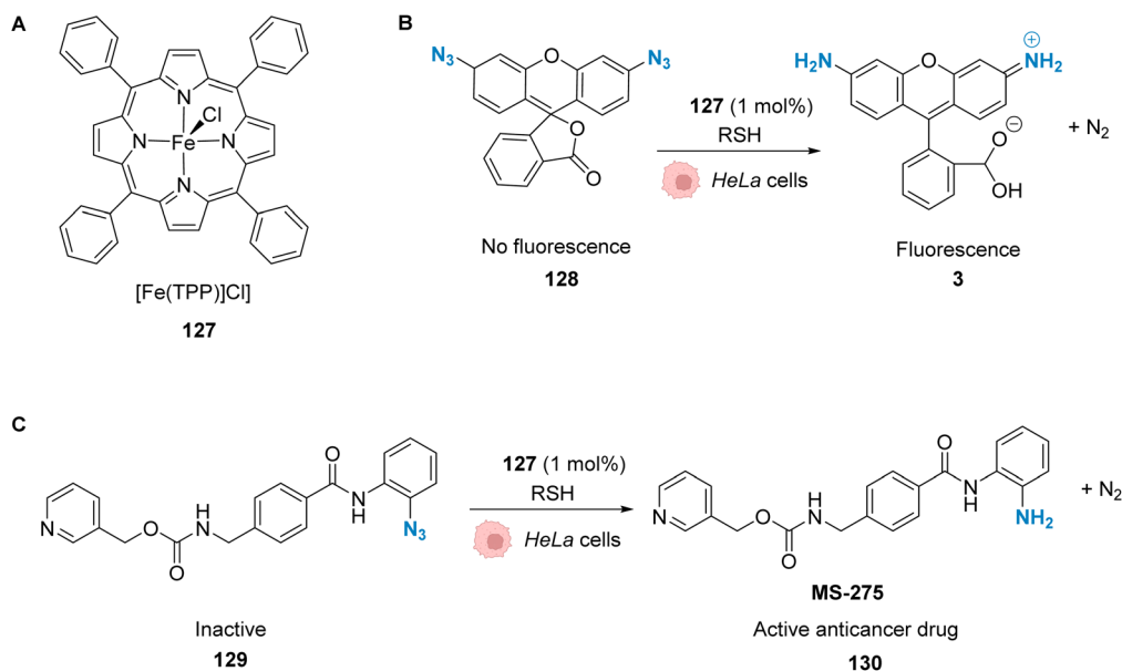
Fig. 43 (A) Structure of a 5,10,15,20-tetraphenyl-21 H ,23 H -porphine (TPP)-containing complex, [ \text{Fe}(\text{TPP})\text{Cl} ]. (B) Iron-mediated reduction of a rhodamine 110 derivative to form fluorescent rhodamine 110. (C) Reduction of the azide molecule 129 to the anticancer drug candidate MS-275. 104
