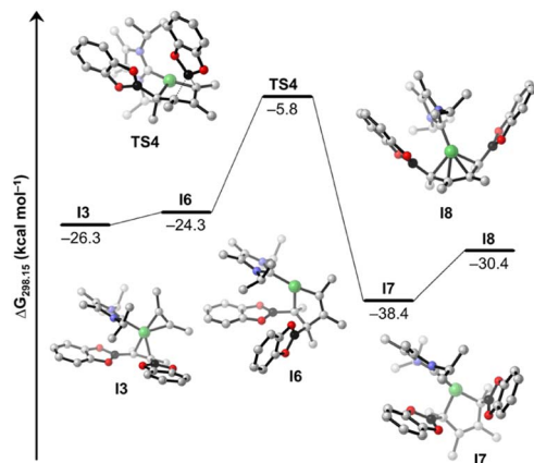
Fig. 6 Free energy profile of the proposed mechanistic pathway from 13 to 18 . Calculated free energies (kcal mol -1 ) are at the SMD(benzene)/PBE0-D3(BJ)/def2-TZVPP//PBE0-D3(BJ)/def2-SVP/def2-TZVP(Ni) level of theory, and are referenced to the resting state 14a + C 2 Me 2 + B 2 cat. Hydrogen atoms are omitted for clarity.
