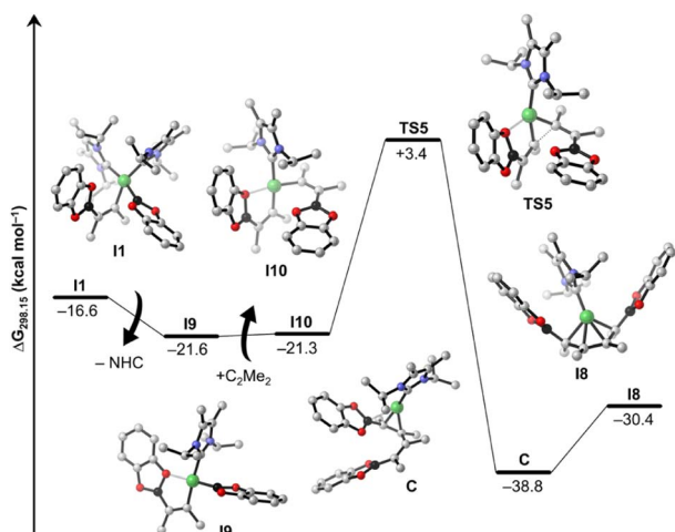
Fig. 7 Free energy profile of the proposed mechanistic pathway from I1 to I8 . Calculated free energies (kcal mol -1 ) are at the SMD(benzene)/PBE0-D3(BJ)/def2-TZVPP//PBE0-D3(BJ)/def2-SVP/def2-TZVPP(Ni) level of theory, and are referenced to the resting state 14a + C 2 Me 2 + B 2 cat 2 . Hydrogen atoms are omitted for clarity.
