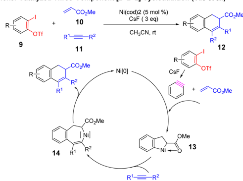
b. Nickel-Catalyzed Three-Component [2+2+2] Cycloaddition (Xie et al.)
