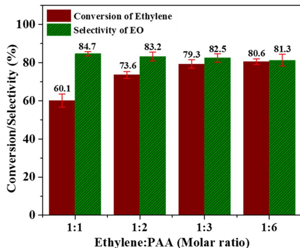
Fig. 7 Effect of ethylene to PAA molar ratio; [reaction conditions: ethylene = 3.28 mmol, catalyst amount = 0.3 g, time = 6 h, solvent = \text{C}_2\text{H}_3\text{N} (20 mL), temperature = 60 °C].
