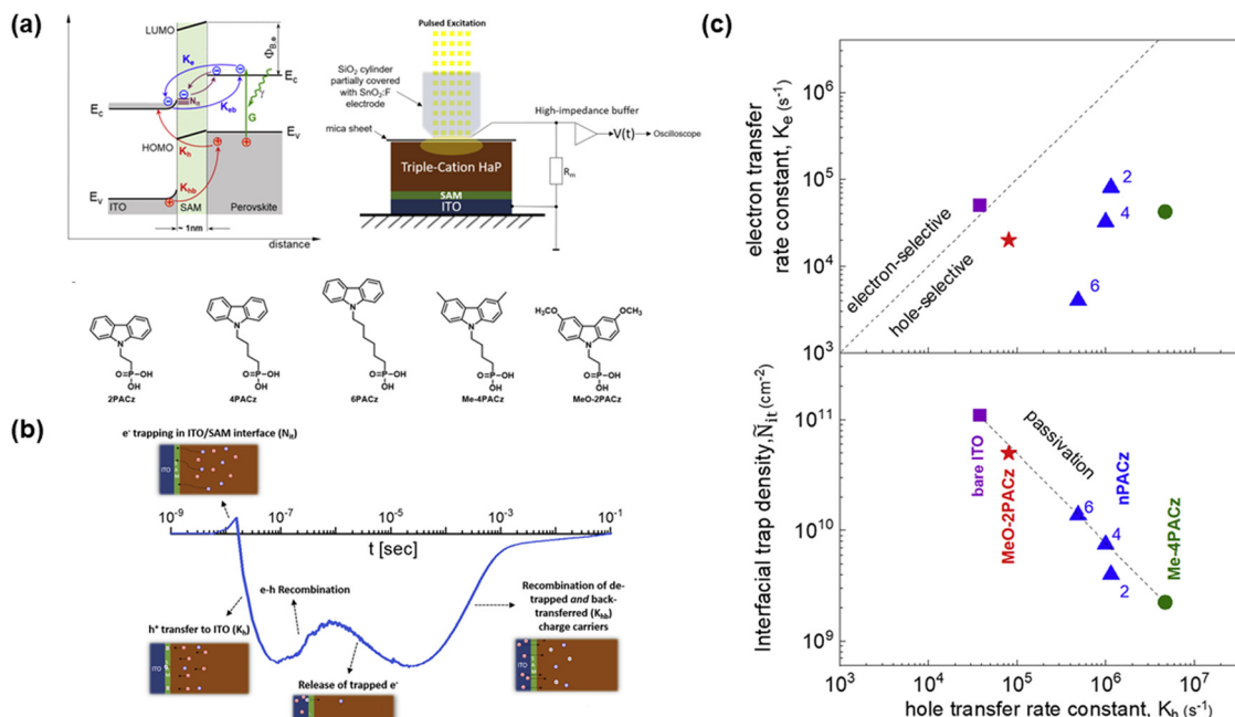
Fig. 3 (a) Schematic model and experimental system for SPV and molecular structure of different SAMs. (b) Timescale of various charge transfer and charge recombination. (c) Hole vs electron transfer rate constant and corresponding interfacial trap density for different SAMs. Reproduced with permission. 39 Copyright 2021, Cell Press.
