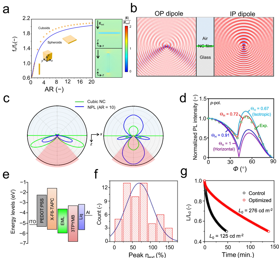
Fig. 6 (a) Calculated ratio of horizontal (x) to vertical (z) local field factor, f_x/f_z , as a function of the aspect ratio. Calculated electric field intensity profiles (b) and radiation patterns (c) in the x-z plane for an out-of-plane (OP; left) and in-plane (IP; right). (d) Angle-dependent PL. (e) Schematic illustration of PeLEDs, and (f and g) optoelectronic properties of PeLEDs. Reproduced with Permission. 79 Copyright 2022, Nature Publishing Group.
