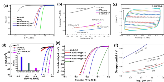
Fig. 7 (a) Linear sweep voltammograms of Er-MOF/MoS 2 , MoS 2 , and Er-MOF, in 0.5 M H 2 SO 4 at a scan rate of 5 \text{ mV s}^{-1} . (b) The corresponding Tafel plots of Er-MOF/MoS 2 , MoS 2 . (c) Cyclic voltammetry of Er-MOF/MoS 2 in the non-Faraday potential region at different scanning rates in 0.5 M H 2 SO 4 . Copyright 2022, Elsevier. (d) Polarization curves of carbon cloth (CC), ZIF-8/CC, CoP-C/CC, CeO 2 -CoP-C/CC, and Pt/C in a N 2 -saturated 0.5 M H 2 SO 4 solution. Scan rate: 2 \text{ mV s}^{-1} . Inset shows the corresponding overpotential of CoP-C/CC, CeO 2 -CoP-C/CC, and Pt/C at the current density of 10 \text{ mA cm}^{-2} ( j_{10} ). Copyright 2018, Elsevier. (e) Polarization curves of HER, Copyright 2021, Wiley VCH. (f) The corresponding Tafel plots for HER, Copyright 2021, Wiley VCH.
