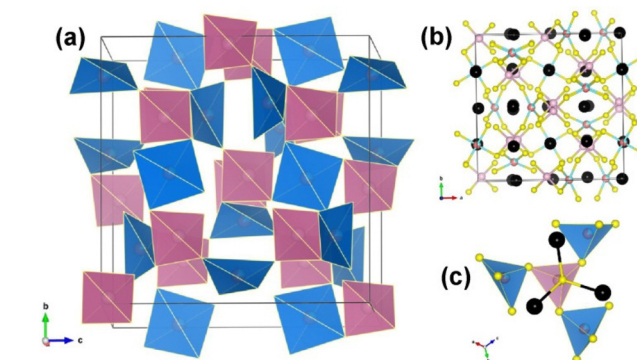
Fig. 13 Crystal structural of \text{Ba}_6\text{Cu}_{1.9}\text{Mg}_{1.1}\text{Sn}_4\text{S}_{16} : (a) polyhedral packing model; (b) ball-and-stick model; (c) coordination environment of [(\text{Cu}/\text{Mg})\text{S}_4] (pink) and [\text{SnS}_4] (blue) tetrahedra. Black: Ba; red: Mg; blue: Cu; pink: Sn; yellow: S. Copyright 2021 American Chemistry Society.
