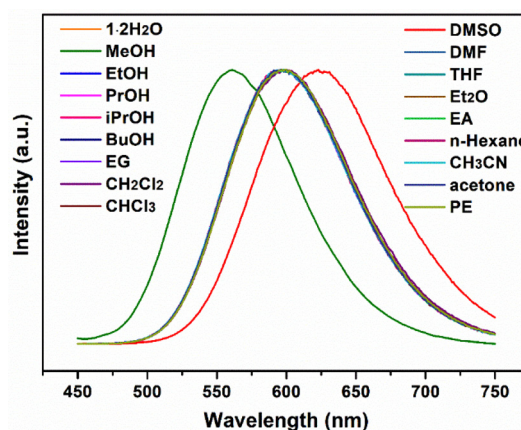
Fig. 6 Emission spectra of 1 \cdot 2\text{H}_2\text{O} on exposure to MeOH, \text{EtOH} , \text{PrOH} , \text{iPrOH} , \text{BuOH} , \text{EG} , \text{CH}_2\text{Cl}_2 , \text{CHCl}_3 , \text{DMSO} , \text{DMF} , \text{THF} , \text{Et}_2\text{O} , \text{EA} , n -hexane, \text{CH}_3\text{CN} , acetone and \text{PE} under 340 nm excitation.
