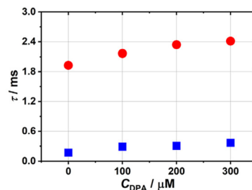
Fig. 7 The lifetimes of 4 in \text{H}_2\text{O} and \text{D}_2\text{O} with different DPA concentrations (blue dots represent the \text{H}_2\text{O} system and red dots represent the \text{D}_2\text{O} system).
