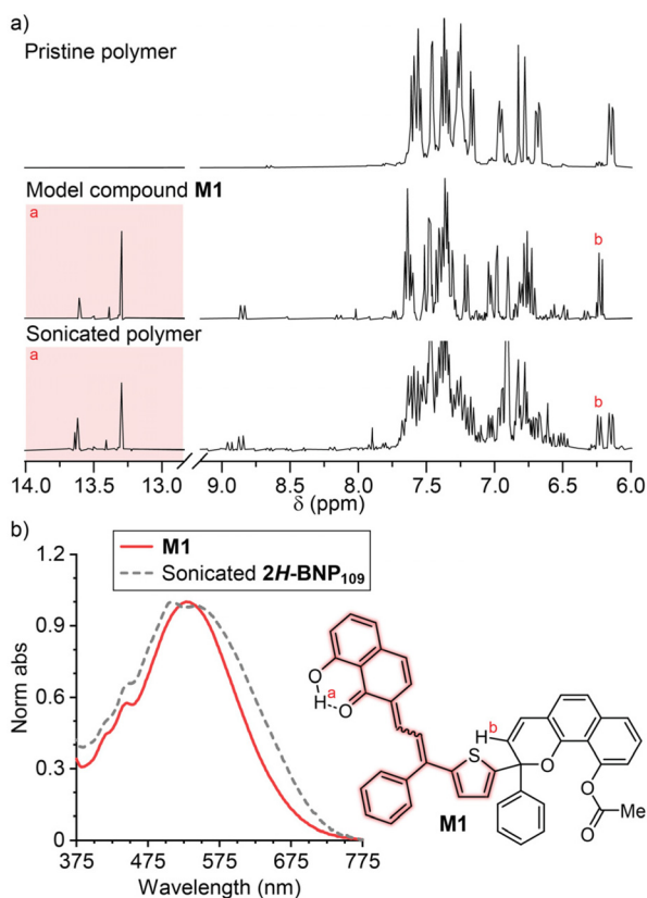
Fig. 3 (a) Characteristic resonances in the ^1\text{H} NMR ( \text{THF-}d_6 , 400 MHz) spectrum of model compound M1 are also observed in the product mixture generated from ultrasound-mediated mechanical activation of 2H-BNP 109 . (b) The absorption spectrum generated upon ultrasonication of 2H-BNP 109 is bathochromically shifted compared to the absorption spectrum of M1 .
