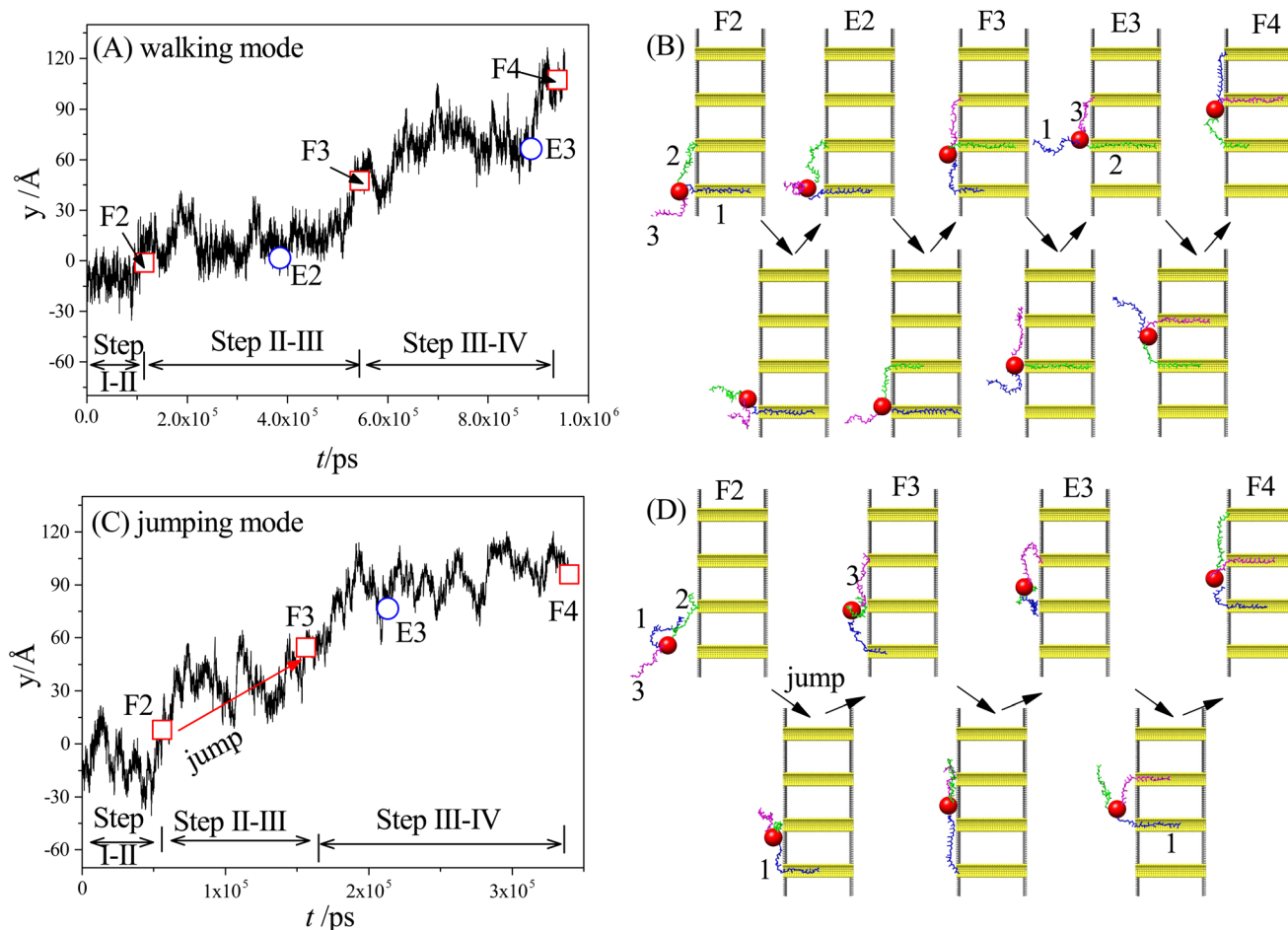
Fig. 3 (A and B) The time-evolutional trace along the y-direction (A) and the snapshots of the nanorobot states (B) for the walking mode. (C and D) The time-evolutional trace (C) and the corresponding snapshots of the nanorobot states (D) for the jumping mode. The leg1, leg2, and leg3 are colored in blue, green, and magenta, respectively. The states F2, F3, and F4 represent the moments when the ssDNA legs of nanorobot find the pore II, III, and IV, respectively, for the first time. The states E2 and E3 represent the moments that the legs enter the pore II and III, respectively, without retreating. Moreover, the snapshots between the F-states and the E-states represent the mid-states that the nanorobot adjusts its conformation, while the snapshots between the E-states and the F-states show the mid-states that the nanorobot moves forward.
