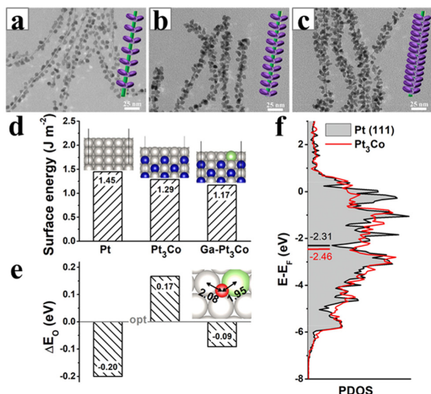
Fig. 28 (a) TEM images and schematic illustrations of (a) 2% Ga-Pt 3 Co, (b) 4% Ga-Pt 3 Co, and (c) 8% Ga-Pt 3 Co nanowires. (d) Surface energy and (e) \Delta E_0 of the pure Pt, Pt 3 Co, and Ga-doped Pt 3 Co (111) surfaces. The optimal E_0 is set to 0. The computational models are shown in insets: gray, blue, green, and red spheres represent Pt, Co, Ga, and O atoms, respectively. (f) The partial density of states (PDOS) for the 3d band of the Pt atoms in the pure Pt and Pt 3 Co surfaces, respectively. The horizontal lines indicate the calculated d-band centres. Reprinted with permission from ref. 76. Copyright 2020 from the American Chemical Society.
