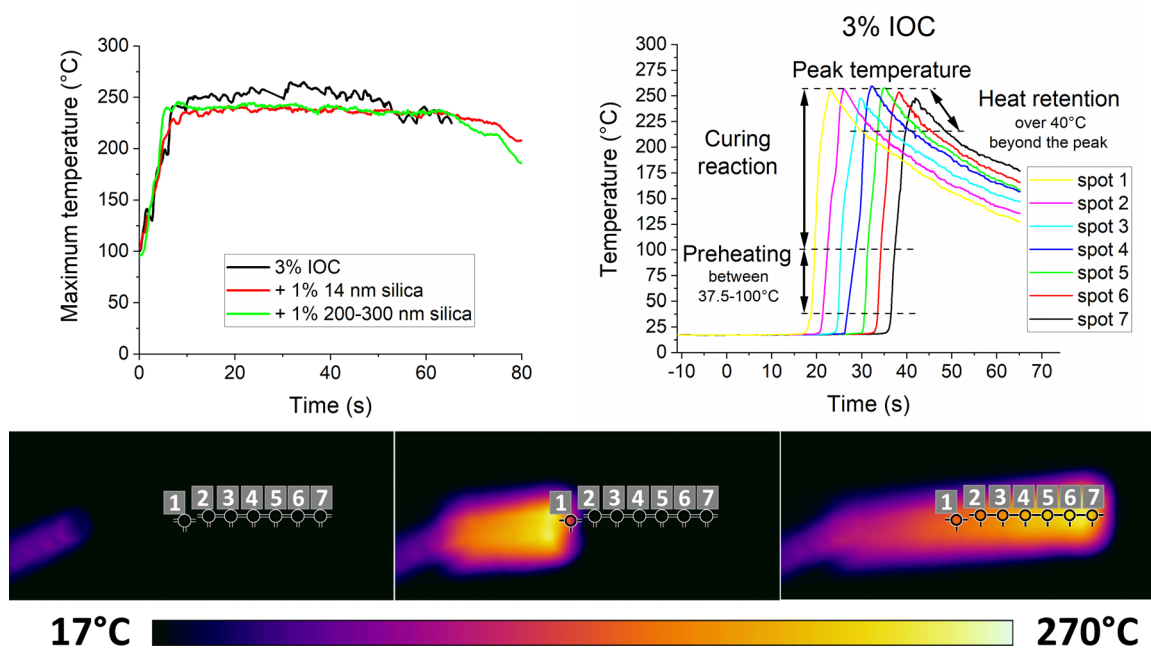
Fig. 4 Maximum temperature (top left) and temperature profiles of the heat unfilled 3% IOC sample at selected fixed points (top right) of the frontal polymerization recorder by thermal imaging (bottom). Temperature profiles of the filled samples can be found in Fig. S5 (ESI†).
